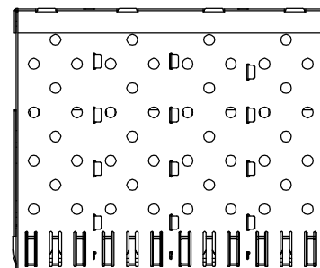
CAGE W/O LIGHT PIPE
